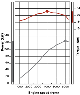
2.4L MIVEC Engine
