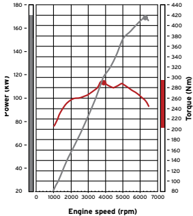
3.0L MIVEC V6 Engine
